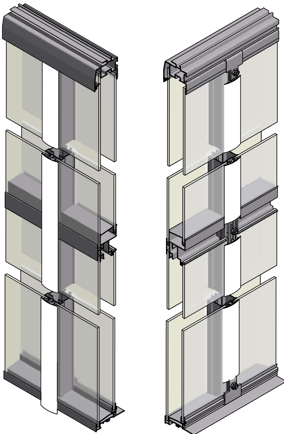
Title: Slimline greenhouse gable system (2x 4mm glass) Slimline kasgevelsysteem (2x 4mm glas)
