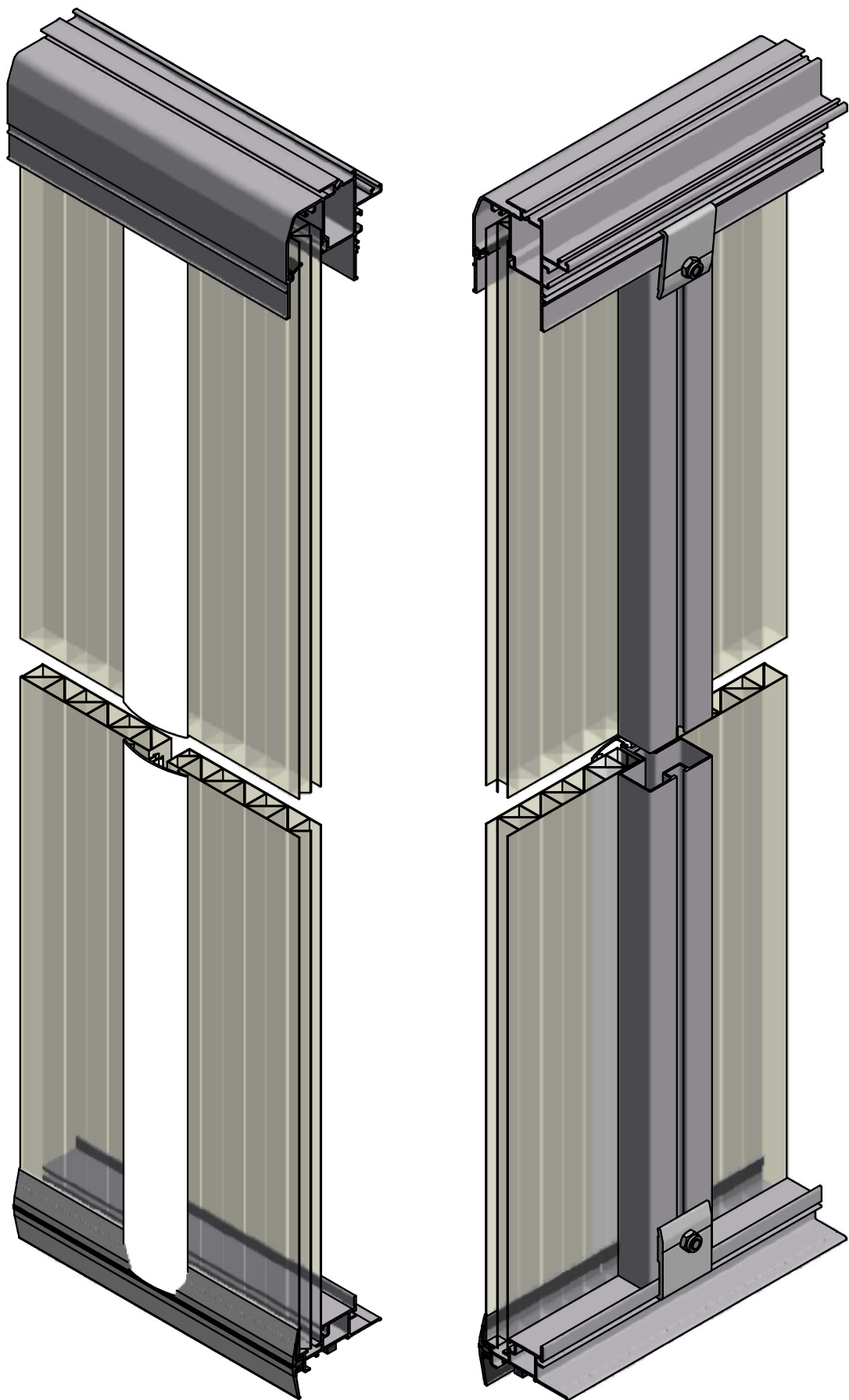
Title: Slimline greenhouse gable system (16mm SDP without panel divider) Slimline kasgevelsysteem (16mm SDP zonder steunregel)
