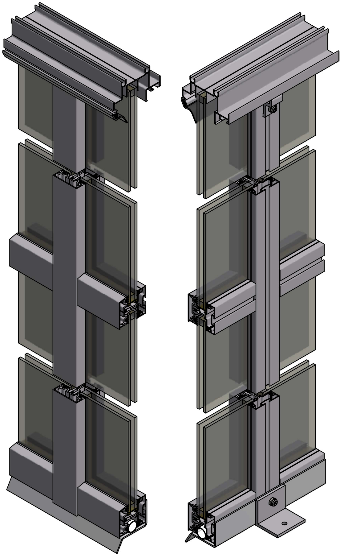
Title: Greenhouse gable system (16mm insulation glass) Kasgevelsysteem (16mm isolatie glas)
