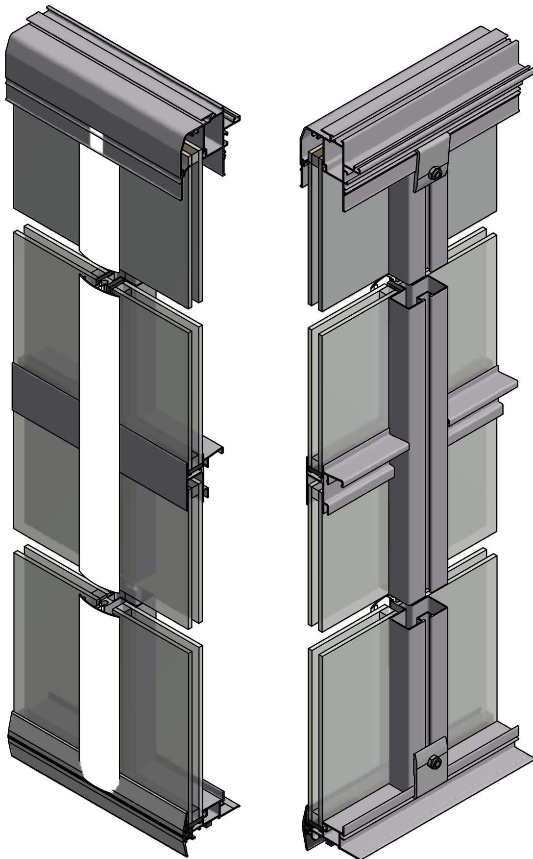
Title: Slimline greenhouse gable system (16mm insulation glass) Slimline kasgevelsysteem (16mm isolatie glas)
